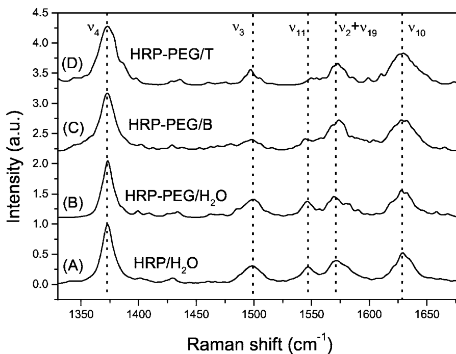
FIGURE 2 Raman spectra (1350–1700 \text{cm}^{-1} ) of native HRP in water (pH 5.6) (A) and HRP-PEG in water (pH 6.5) (B), benzene (denoted as HRP-PEG/B) (C), and toluene (denoted as HRP-PEG/T) (D). In organic solutions, the Raman bands from solvents have been subtracted. For comparison of relative intensities, all spectra are plotted with intensity of \nu_4 normalized to 1.
